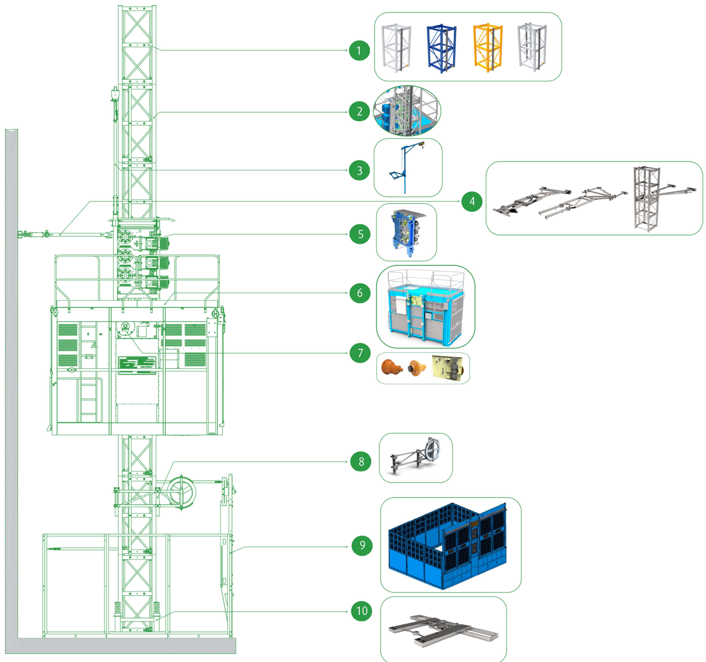
SC Series Construction Hoists Sketch
